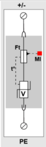
V: High-energy varistor Ft: Thermal fuse t*: Thermal disconnection system MI: Disconnection indicator
